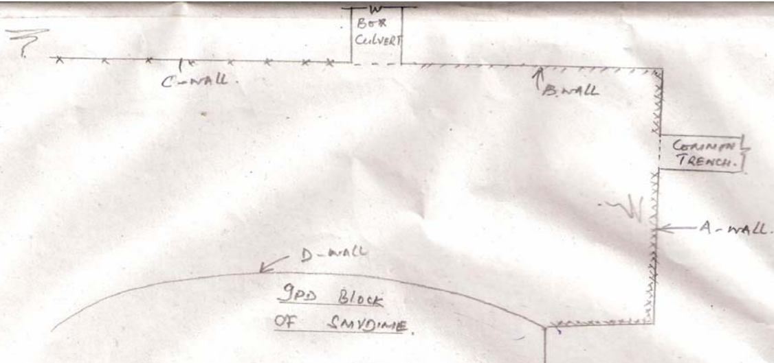
SITE PLAN OF WALLING ON HILLSIDE OF JPD BLOCK BACKSIDE SCALE - NOT TO S
